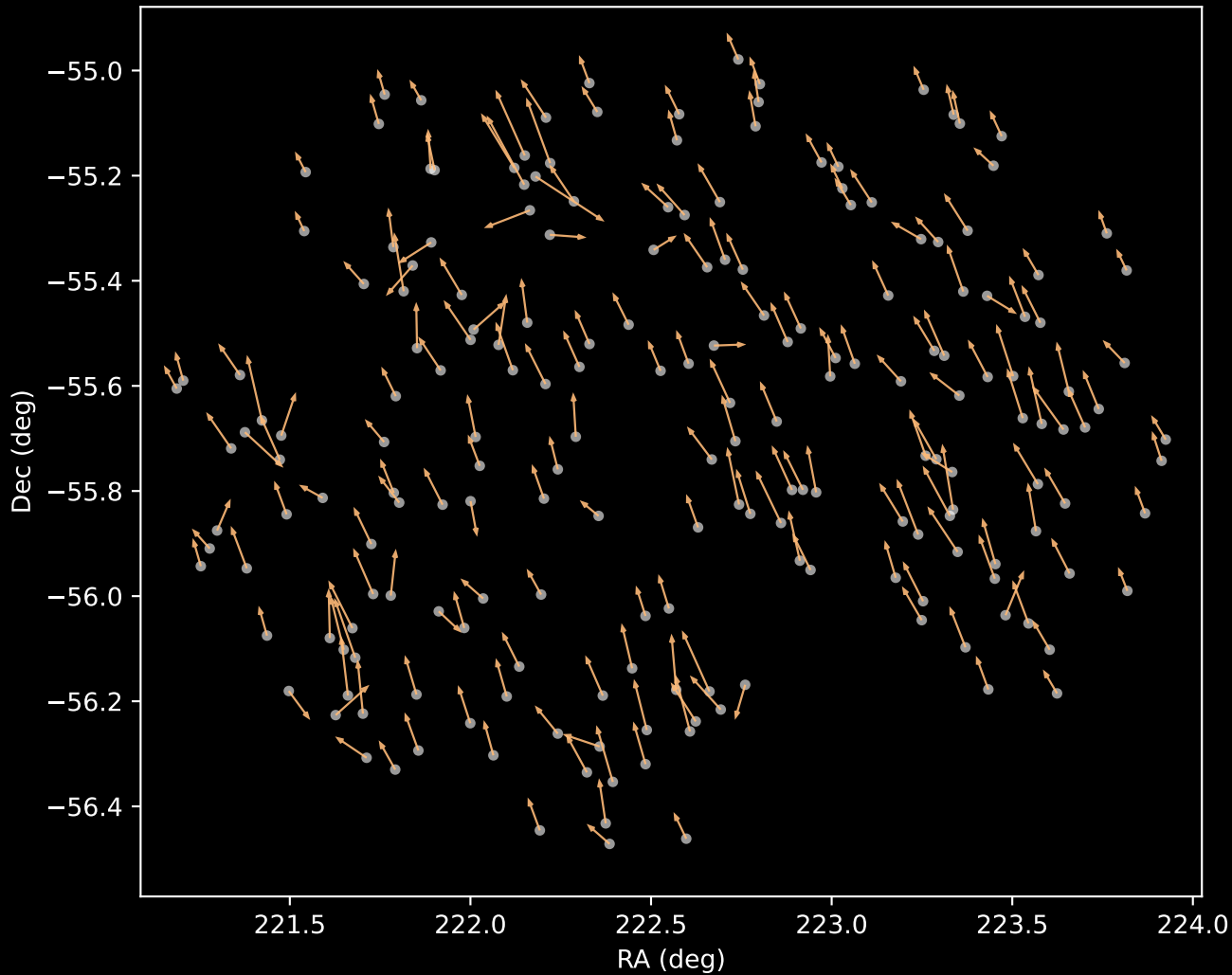
APOGEE DR17 Cluster 3 Proper Motion Vectors (n=201)
