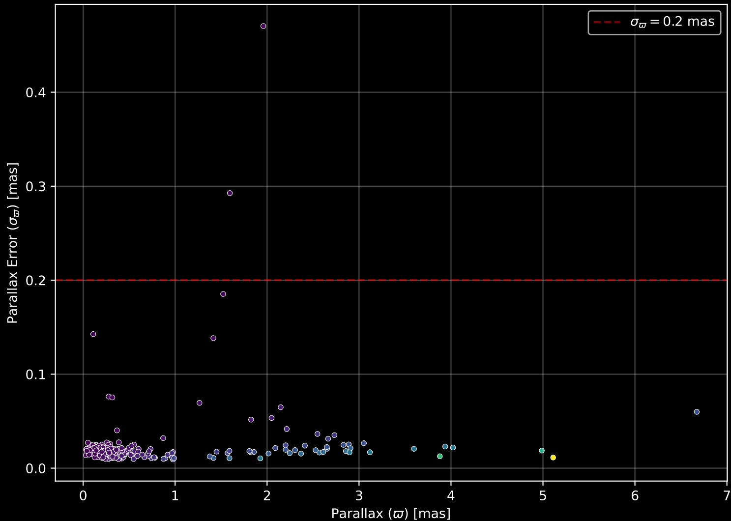
APOGEE DR17 Field: [270-12] Parallax Quality (n= 253)
