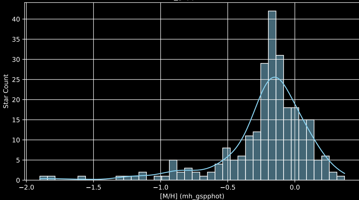
APOGEE DR17 Field: [270-12 [M/H] (mh_gspphot) (n= 253)
