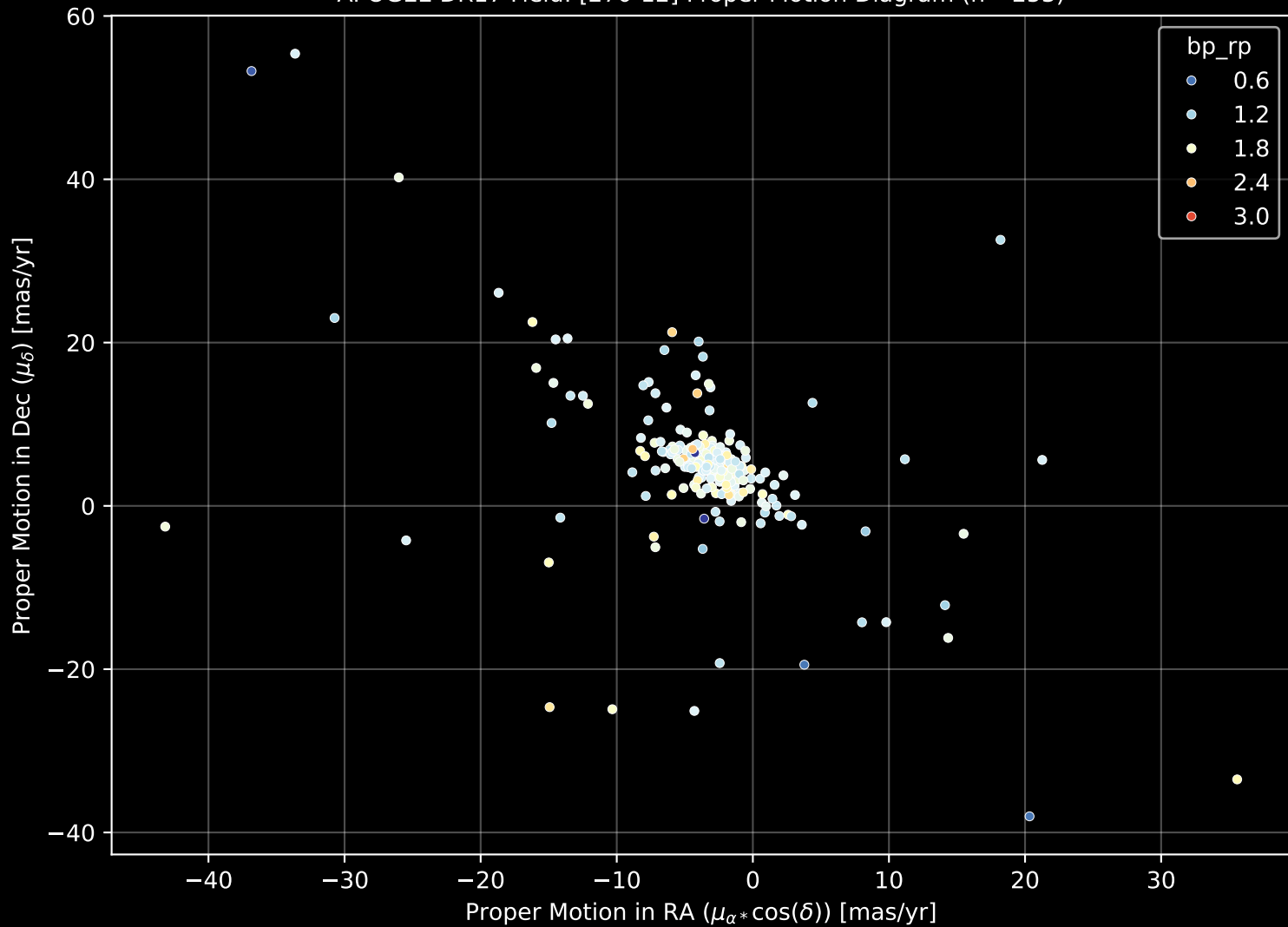
APOGEE DR17 Field: [270-12] Proper Motion Diagram (n= 253)
