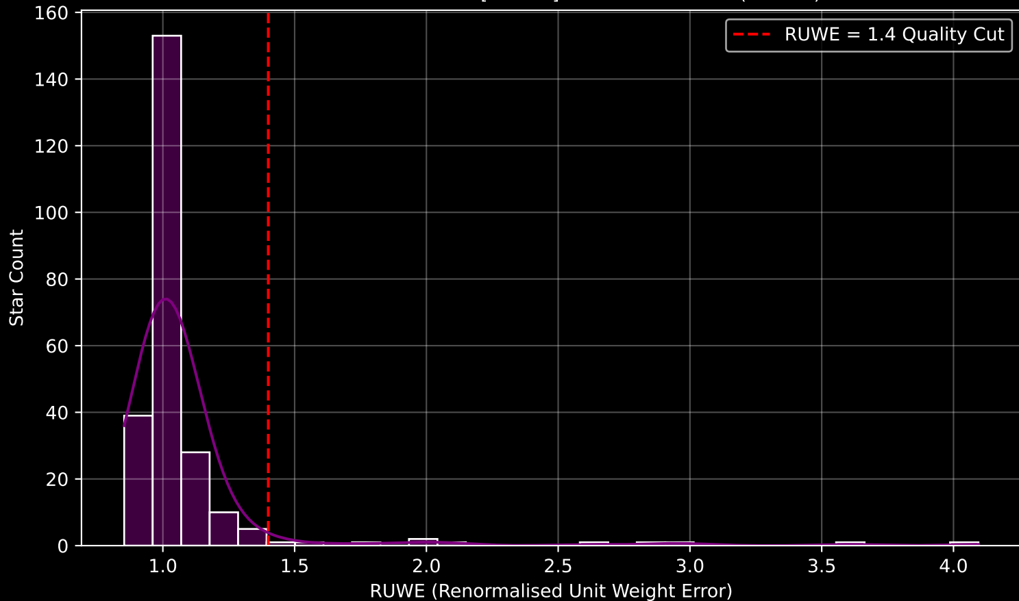
GAPOGEE DR17 Field [270-12] RUWE Distribution (n= 246)
